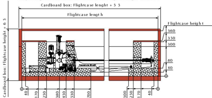
(3) EXAMPLES: Sample-Transporter: MDG40-XXXX=> Flightcase length = XXXX + 715 Sample-Storage: MD40(Y0)-XXXX -RECOMSTACK(D7) H=> Flightcase height = XXXX + 350
