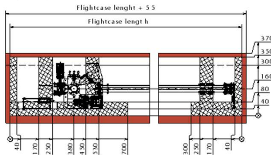
(2) Sample-Transporter: RMD40-XXXX-TSRMVSV => Flightcase length = XXXX + 690 Sample-Storage: no => Flightcase height = standard (360)
