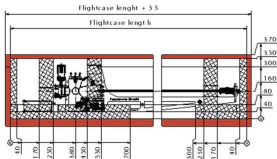
(1) Sample-Transporter: WMG40(FC)-TSWMSNV => Flightcase length = XXXX + 720 Sample-Storage: no => Flightcase height = standard (360)
